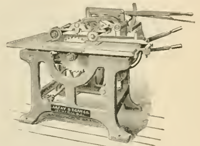
No. 110. NEW SELF FEED RIP SAW
